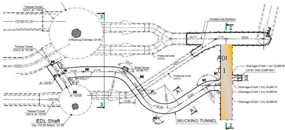
Figure 8 General Layout of ADIT 1 (320 meters)
